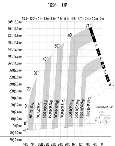
Loading Diagram without Outrigger
