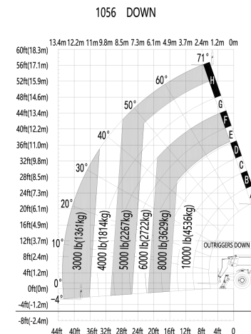
Loading Diagram with Outrigger
